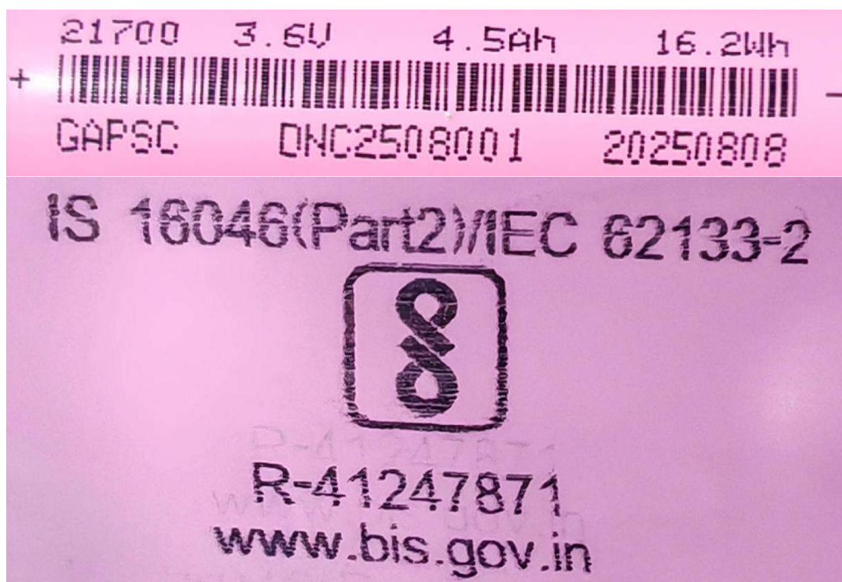
组成电池铭牌 View of the cell nameplate
